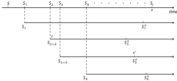
Fig. 2. The destination coloring stochastic process during the spraying phase. destination can be computed observing that the destination is the i -th node encountered by S , and that the random time of this encounter corresponds to the i -th order statistic of random variables S_1, \dots, S_{M-1} . We can then write:
