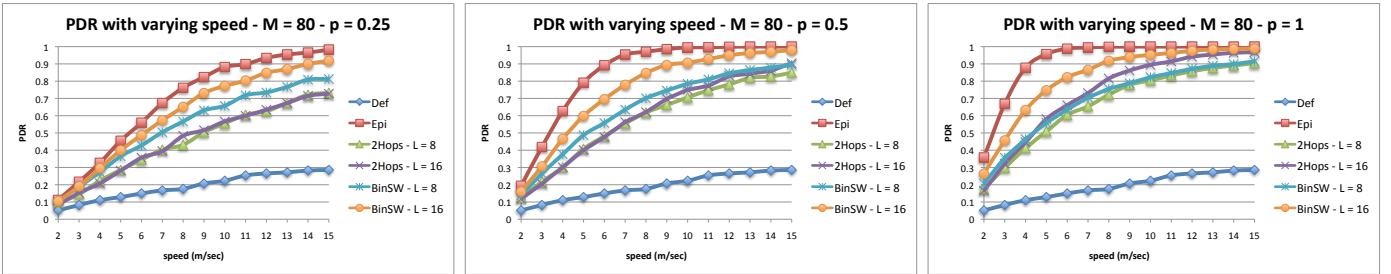
Fig. 7. Probability of correctly delivering a message within time TTL = 3600s with Rand cooperation for RWP mobile networks with M = 80 , with p = 0.25 (left), p = 0.5 (center), and p = 1 (right). For reference, the curve relative to the Def scenario is reported in all graphics.
