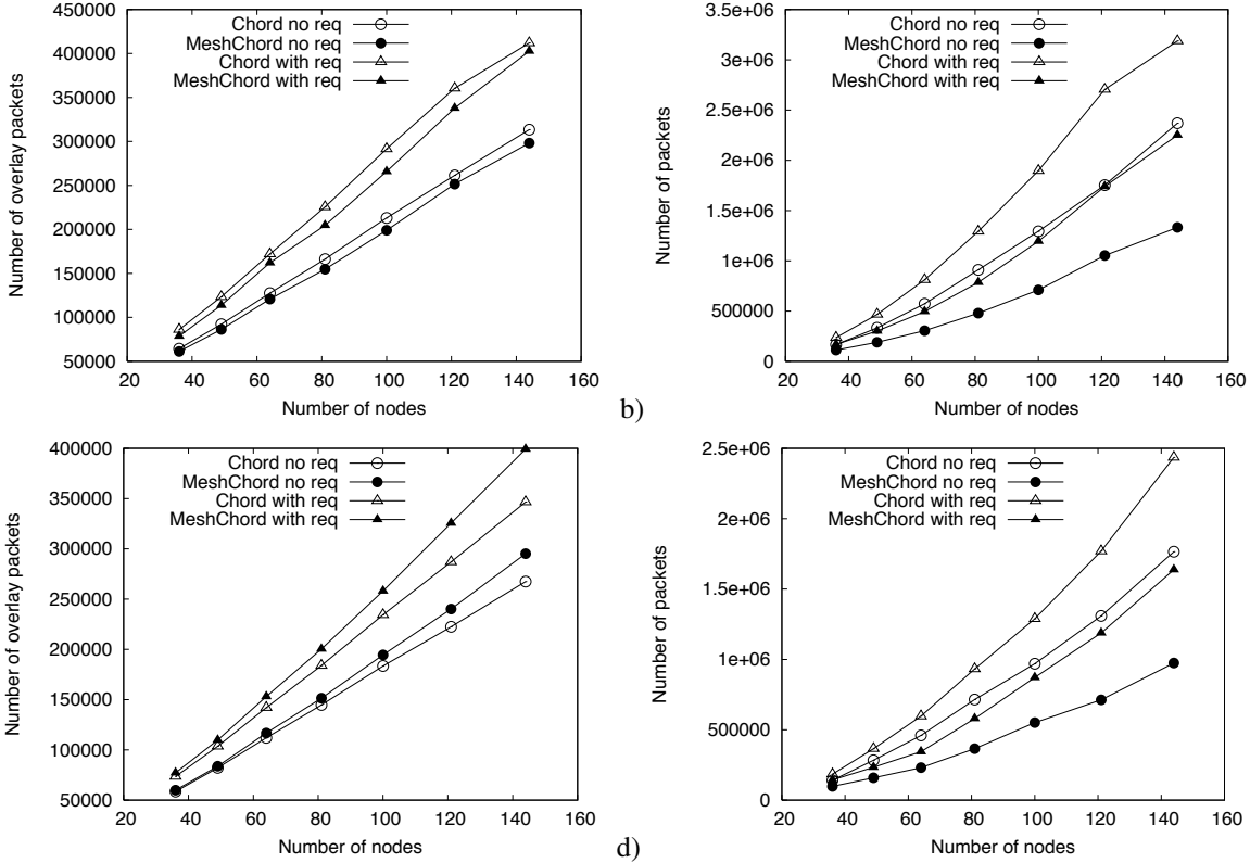
Figure 2. Total number of exchanged overlay-level and network-level packets for different values of n and grid topology: iterative (a-b)) and recursive (c-d)) lookup implementation.
